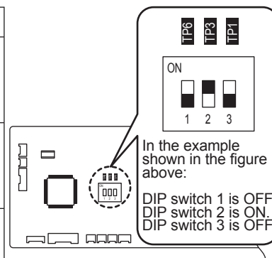
Fig. 1-11-3-8 Indoor unit control PCB
