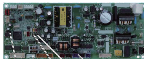
EEPROM TEST pin RC OPTION CHK pin
