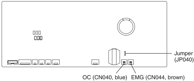
Indoor unit control PCB
