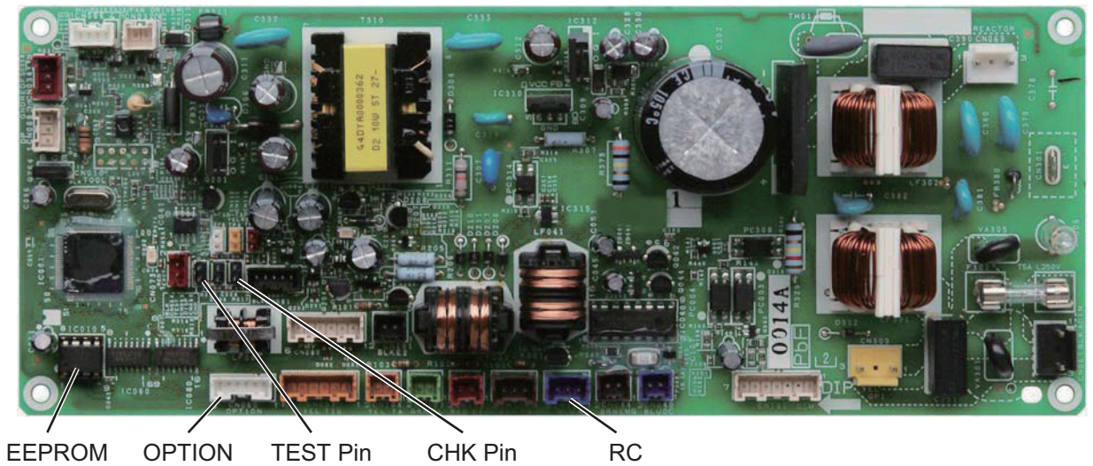
ACXA73-25280 : Duct Type Indoor Unit Control Board
