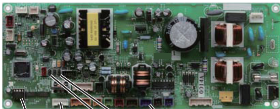
ACXA73-25280 : Duct Type
