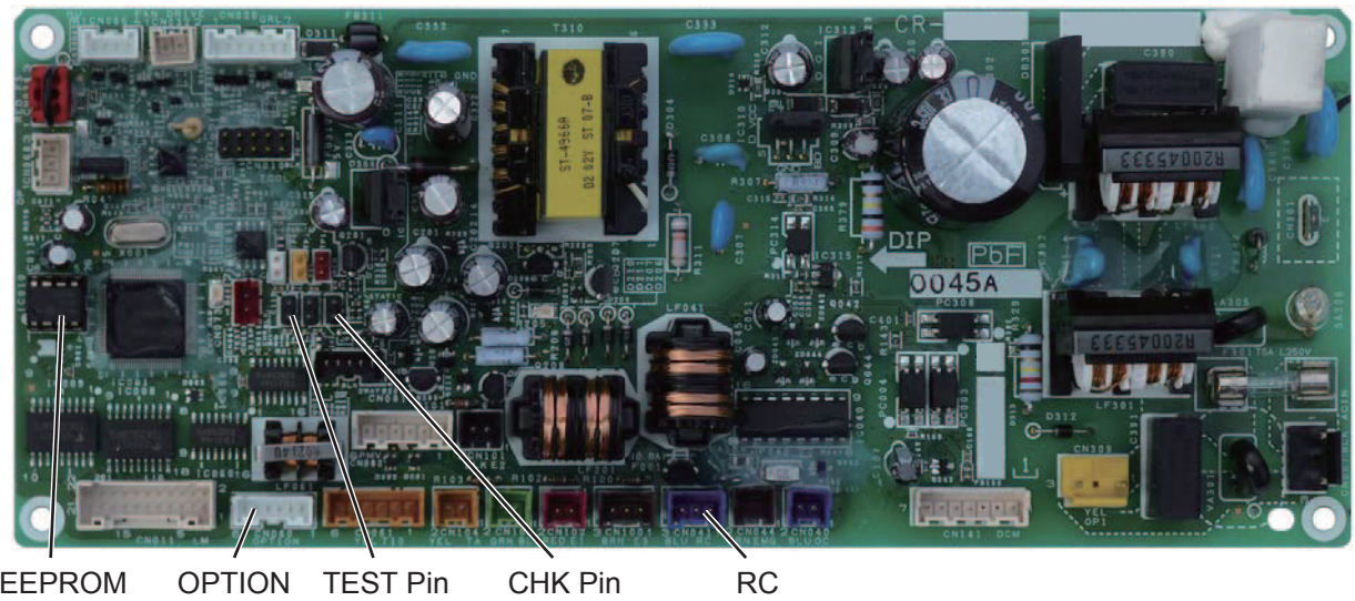
ACXA73-25280 : Duct Type Indoor Unit Control Board
