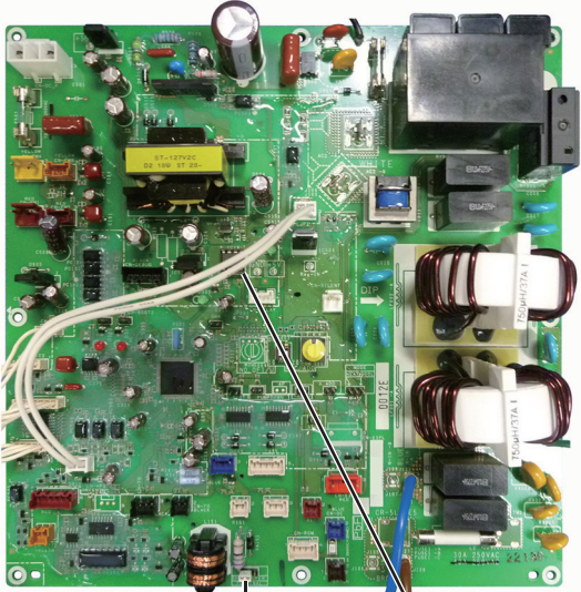
A747895 : (U-100PE1E5A) (for single-phase outdoor unit PCB)
