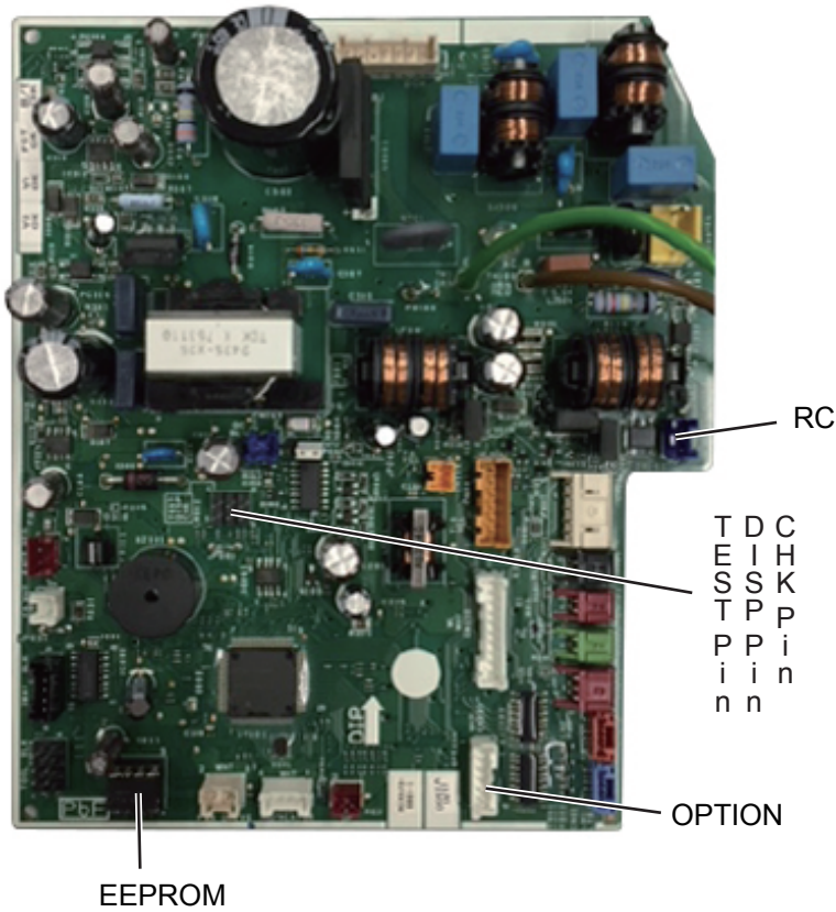
ACXA73C4182 : Wall Mounted Type Indoor Unit Control Board
