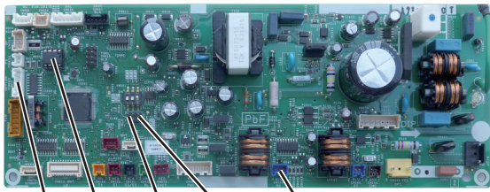
ACXA73-25530 : 4-Way Cassette Type (Type U2)
