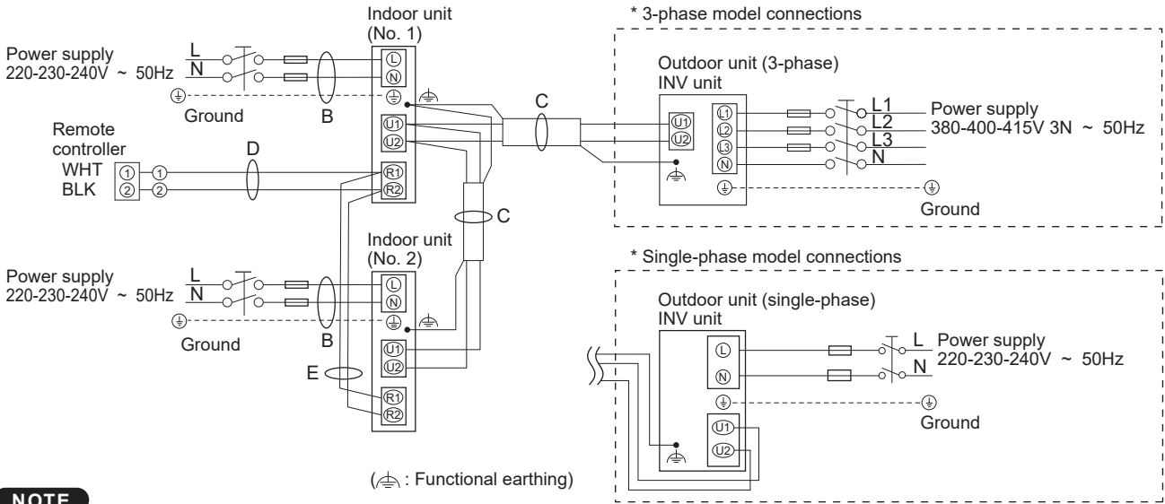
Terminal Board
