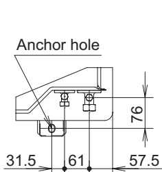
Enlarged view A Refrigerant piping end connection
