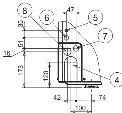
Z VIEW
