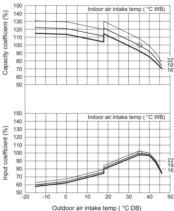
Cooling capacity ratio (maximum capacity)
