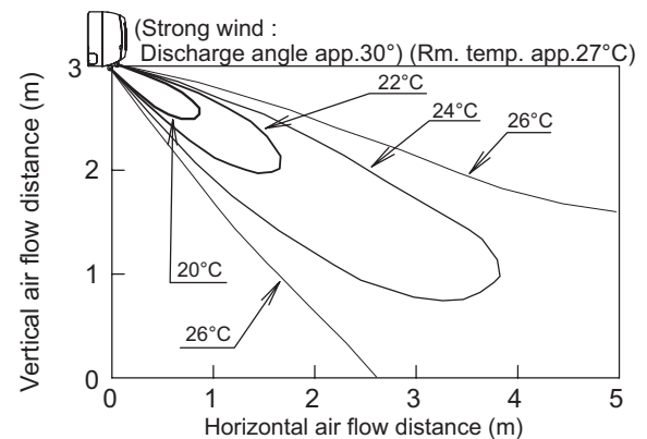
Cooling : Distribution of temperature
