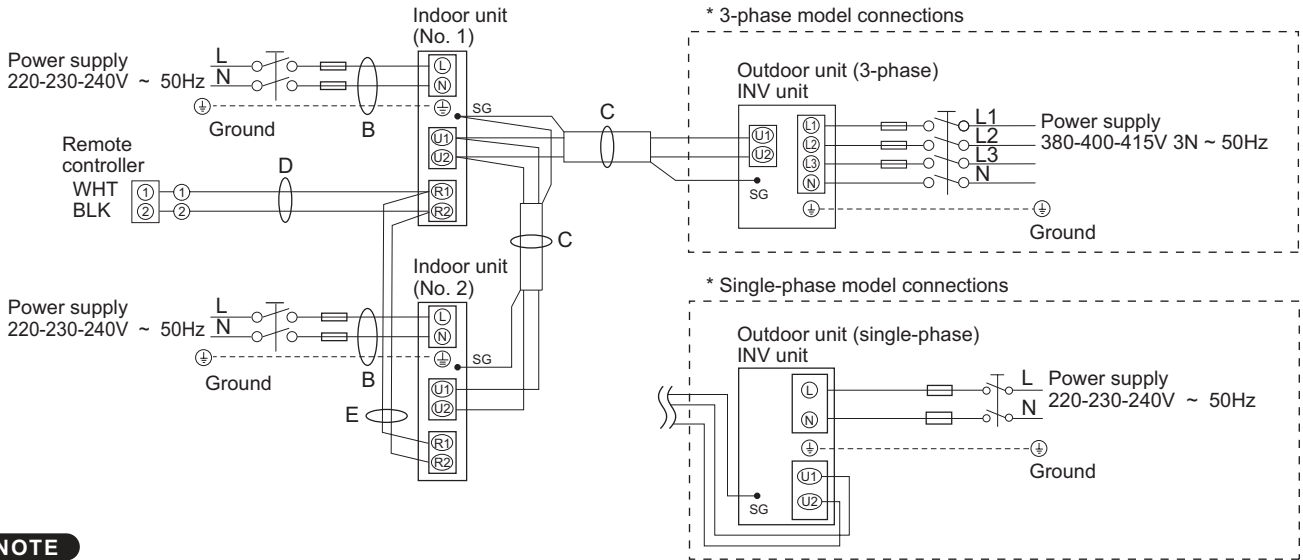
Terminal Board
