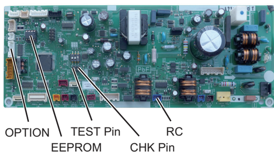
A7302060 : 4-Way Cassette Type (Type U2)
