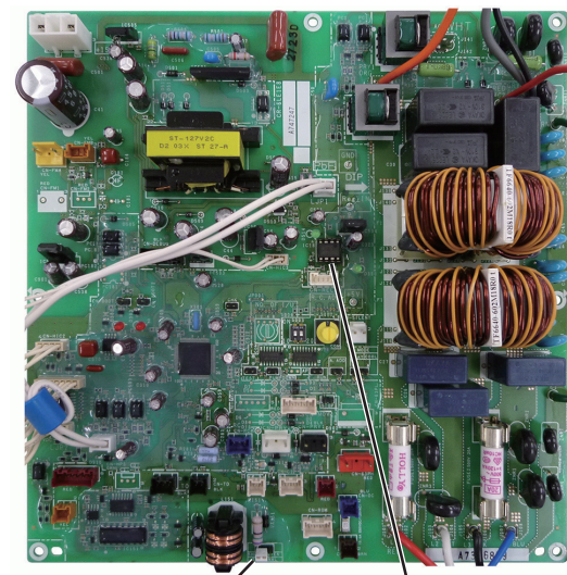
TERMINAL EEPROM
