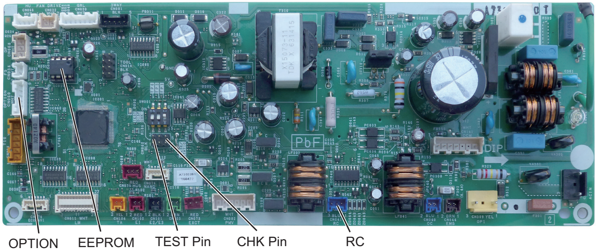
A747931 : Ceiling Type (Type T2) Indoor Unit Control Board
