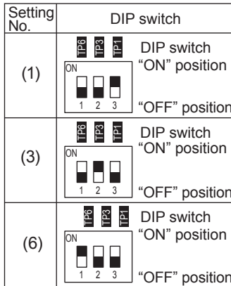
Fig. 1-11-3-3 Indoor unit control PCB
