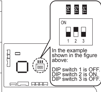
Fig. 1-11-3-8 Indoor unit control PCB
