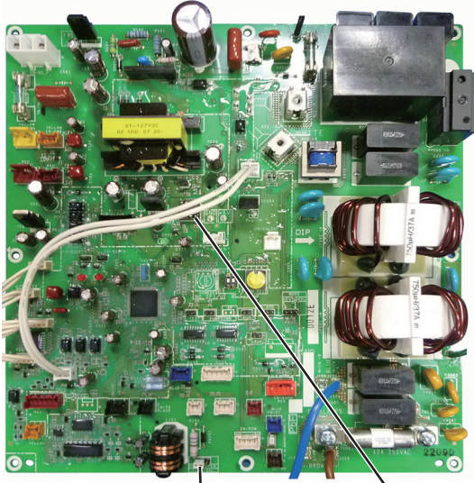
TERMINAL EEPROM
