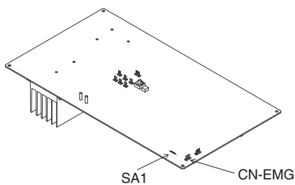
Indoor unit control PCB
