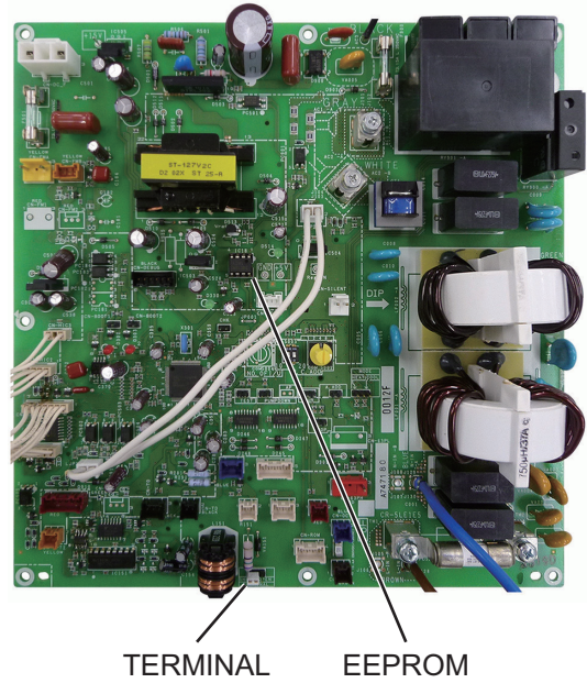
A747180 : (U-125PEY1E5) (for single-phase outdoor unit PCB)
