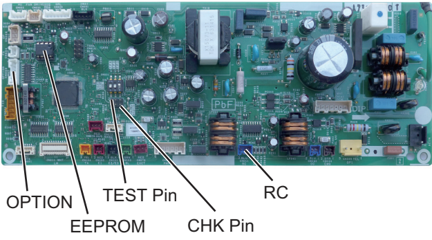
A7302060 : 4-Way Cassette Type (Type U2)
