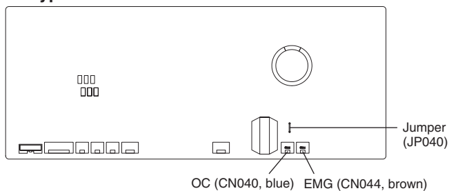
Indoor unit control PCB
