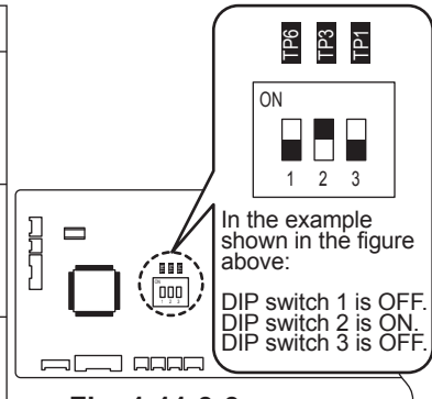
Fig. 1-11-3-3 Indoor unit control PCB
