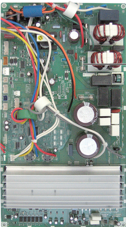
ACXA73-03100 : Bottom side (U-36PE2E5A, U-50PE2E5A, U-60PE2E5A) (U-60PEY2E5, U-71PEY2E5) (for single-phase outdoor unit PCB)
