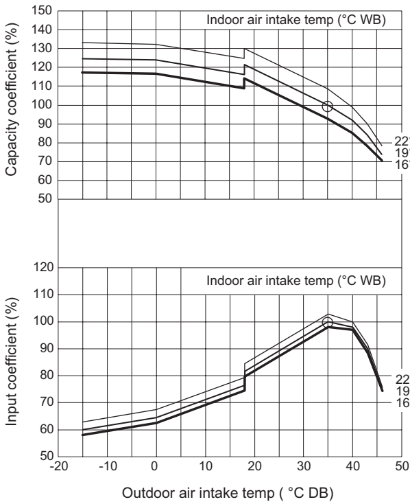
Cooling
