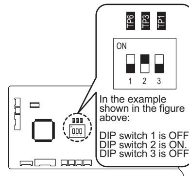
(Fig. 7-7) Indoor unit control PCB
