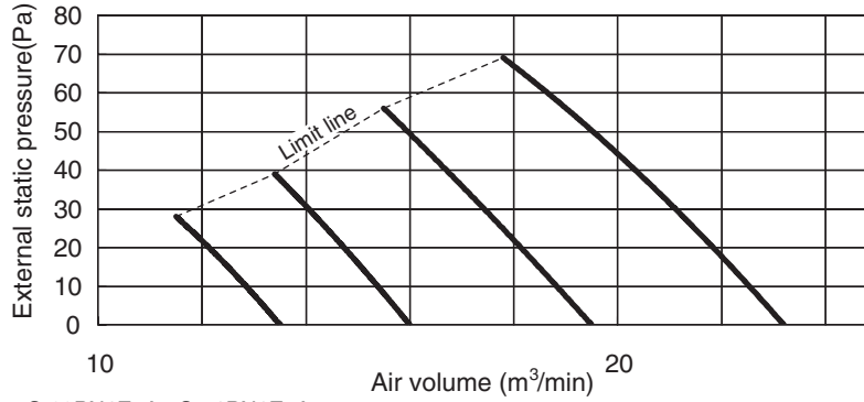
S-60PN1E5A • S-71PN1E5A
