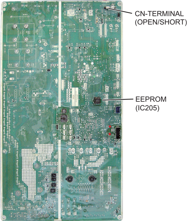
ACXA73-03100 : Up side (U-36PE2E5A, U-50PE2E5A, U-60PE2E5A) (U-60PEY2E5, U-71PEY2E5) (for single-phase outdoor unit PCB)
