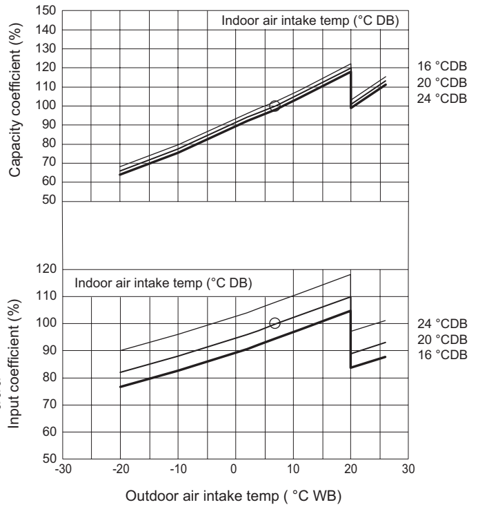
Heating
