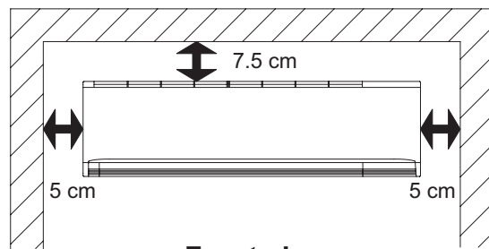
Front view Necessary minimum space for a installation
