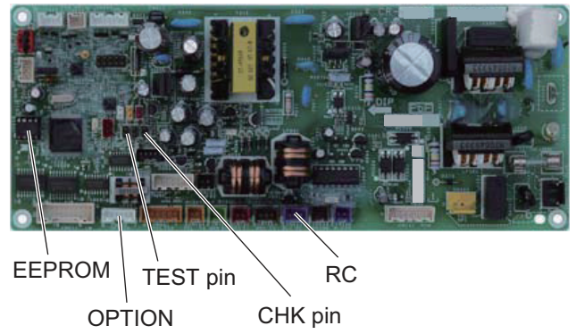
A747931 : Ceiling Type (Type T2)
