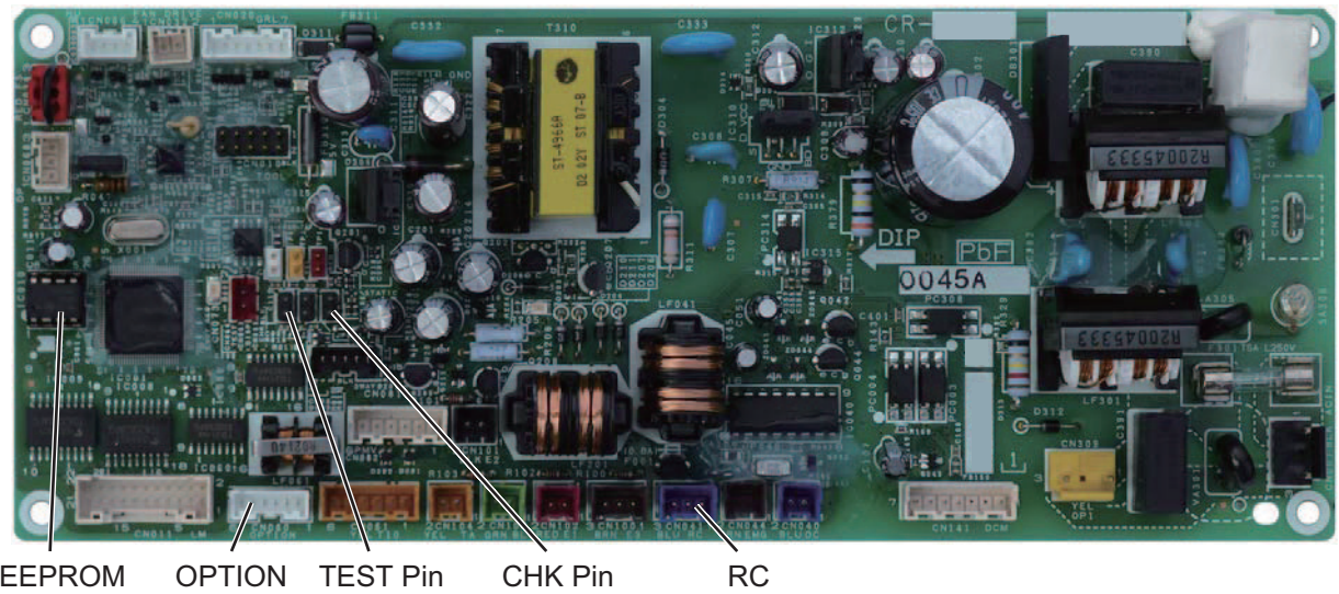
A747938 : Duct Type Indoor Unit Control Board
