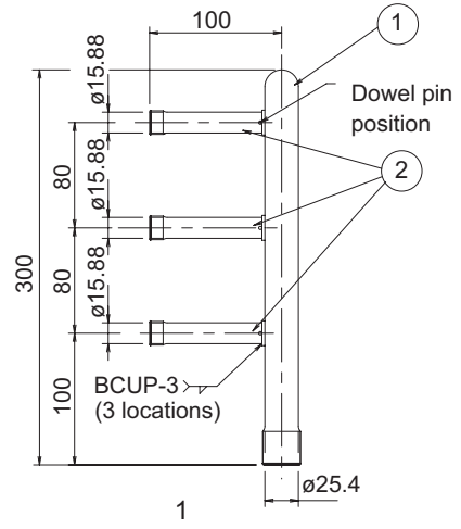
Gas distribution joint for gas tube
