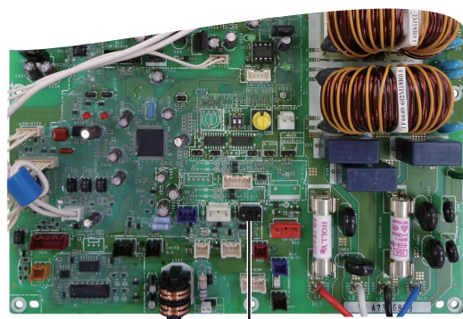
CN-PRY1
