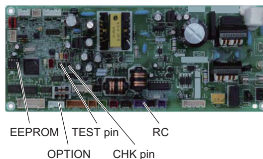
A747931 : Ceiling Type (Type T2)
