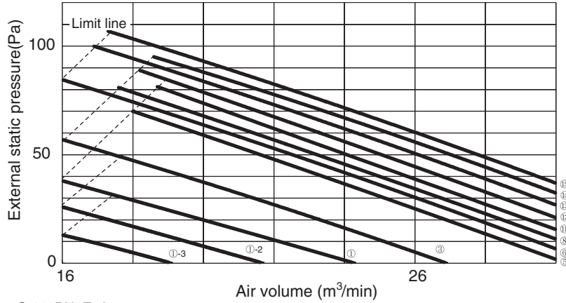
S-100PN1E5A
