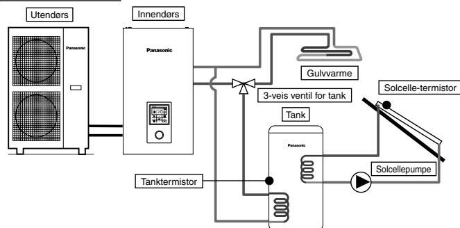
Tank + solcelletilkobling
