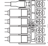
Power supply cable between outdoor and indoor unit
